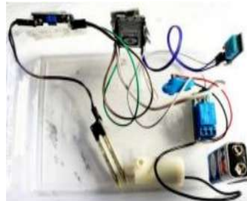
Figure 9: Iot Based Smart Agriculture Monitoring System
