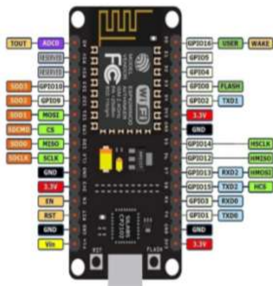
Figure 6: ESP8266 module
