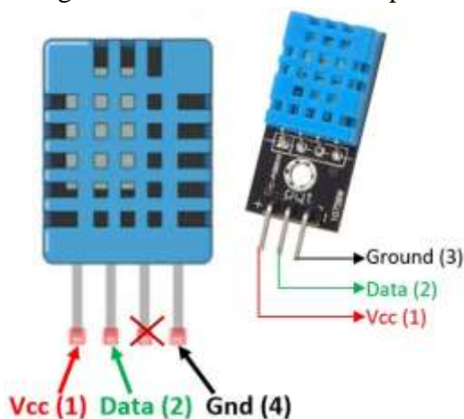
Figure 3: Temperature sensor
